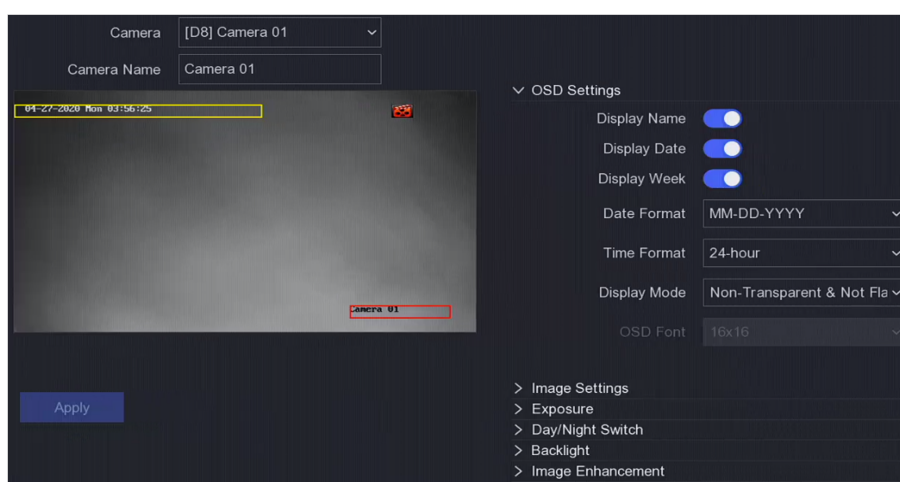
Figure 6-14 OSD
