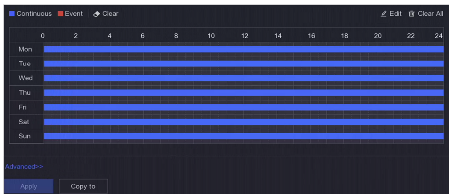
Figure 6-24 Recording Schedule
