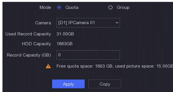
Figure 6-27 Quota
