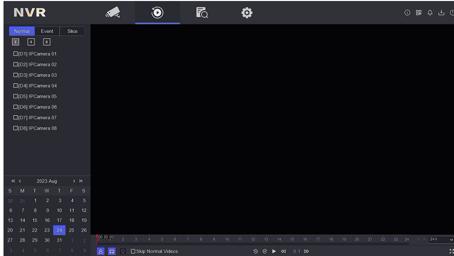
Figure 3-1 Playback
