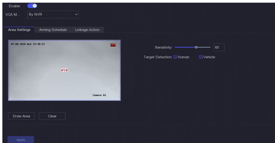
Figure 5-8 Motion Detection
