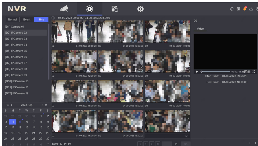
Figure 3-7 Video Slices
