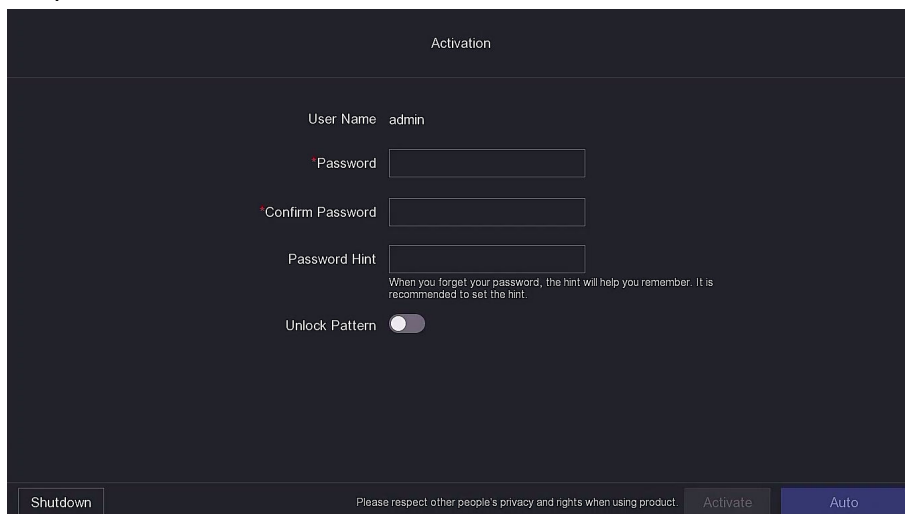
Figure 1-1 Activation
